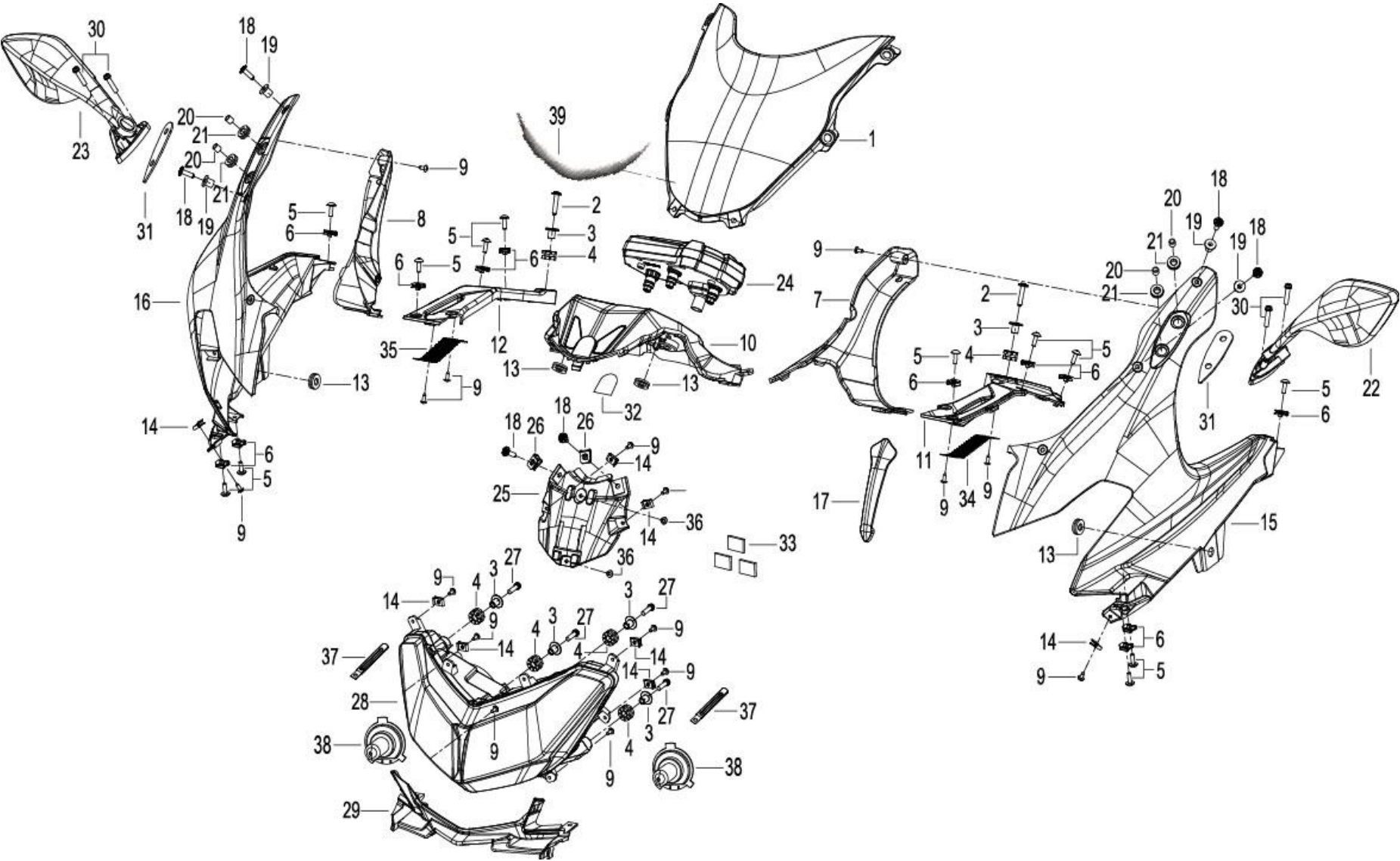
F15 导流罩 BRACKET. ASSY.
