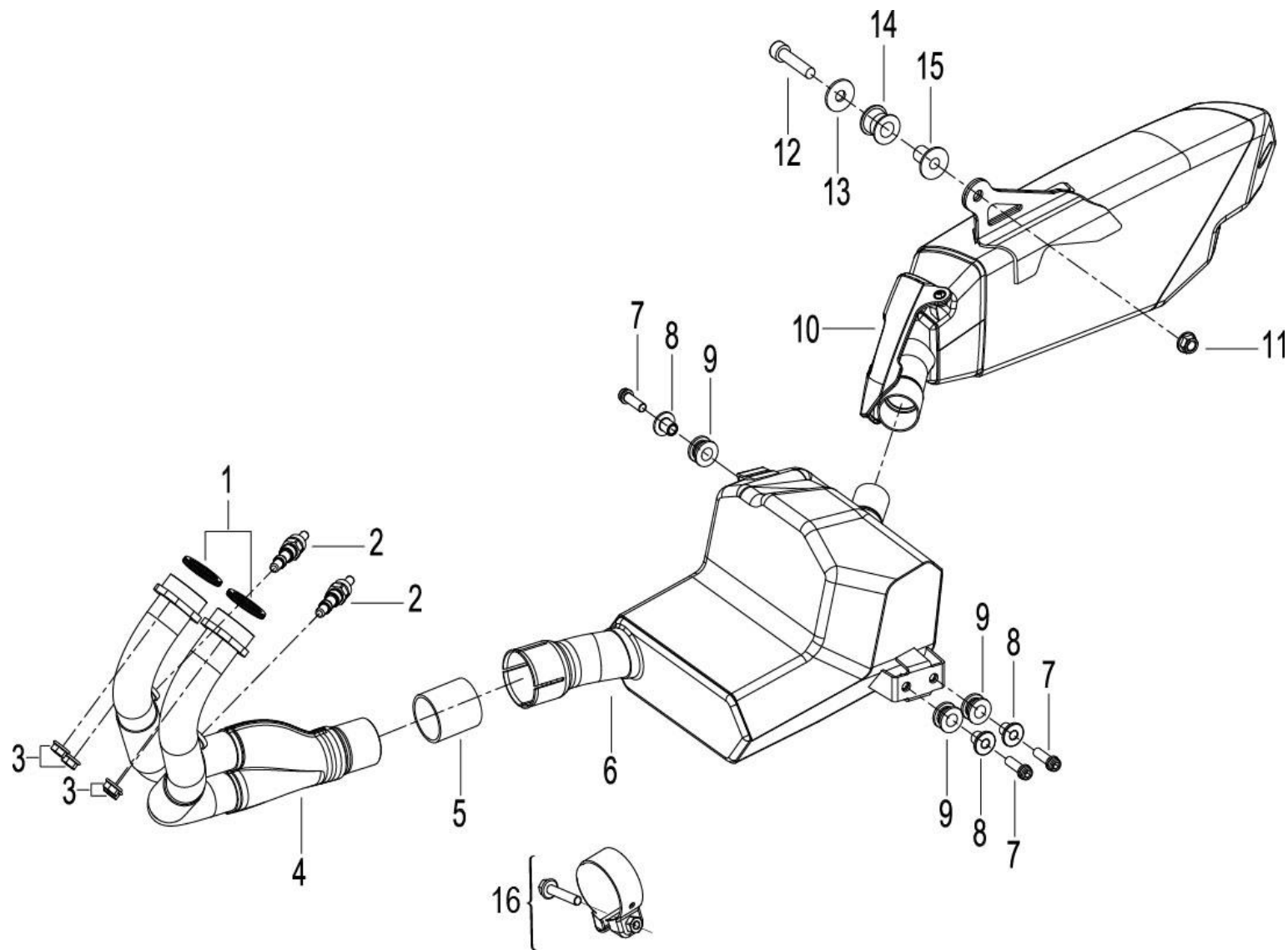
F05 消声器 MUFFLER ASSY.
