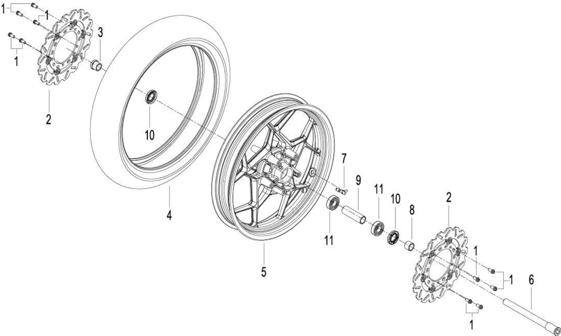
F03 前轮 FRONT WHEEL ASSY.
