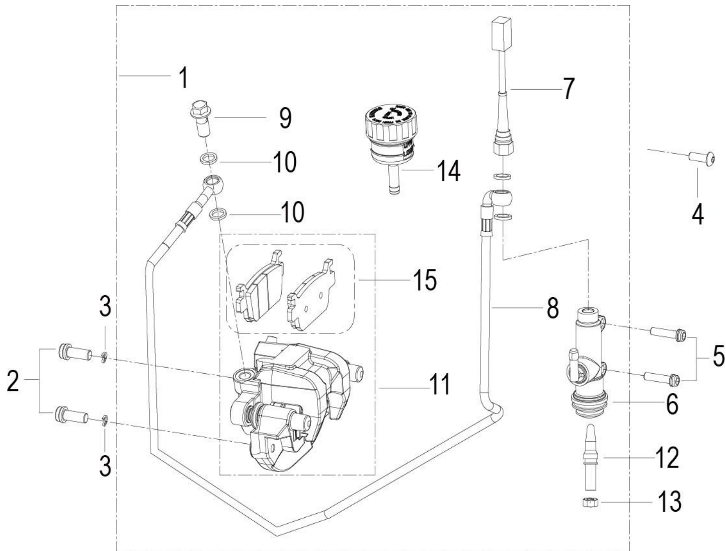
F10 后液刹 REAR DISK BRAKE ASSY.
